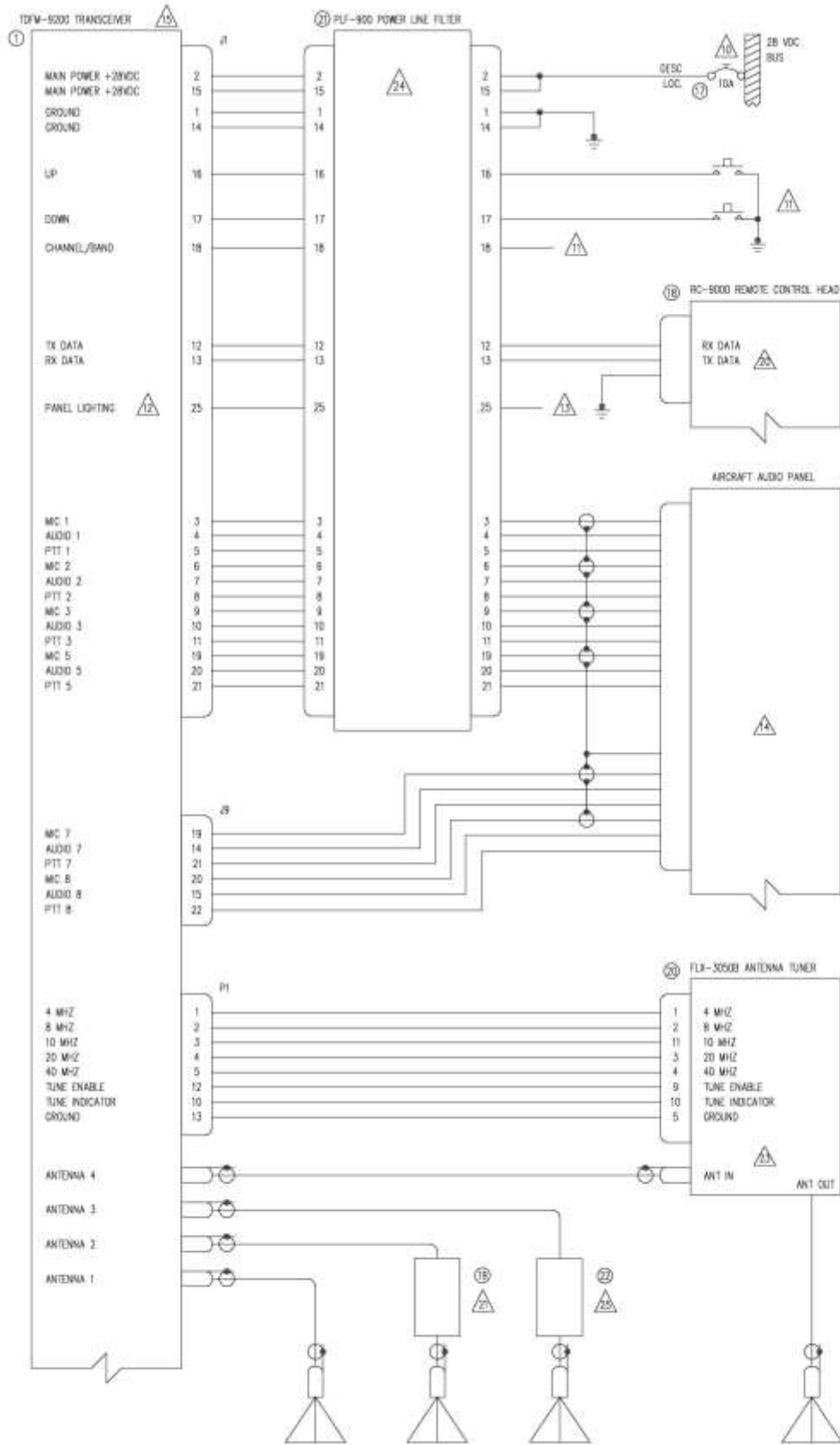
FIGURE 4: Wiring Connections for Individual Band Control.
