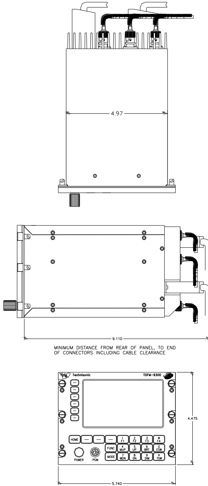
FIGURE 1: Outline Drawing for Model TDFM-9200
