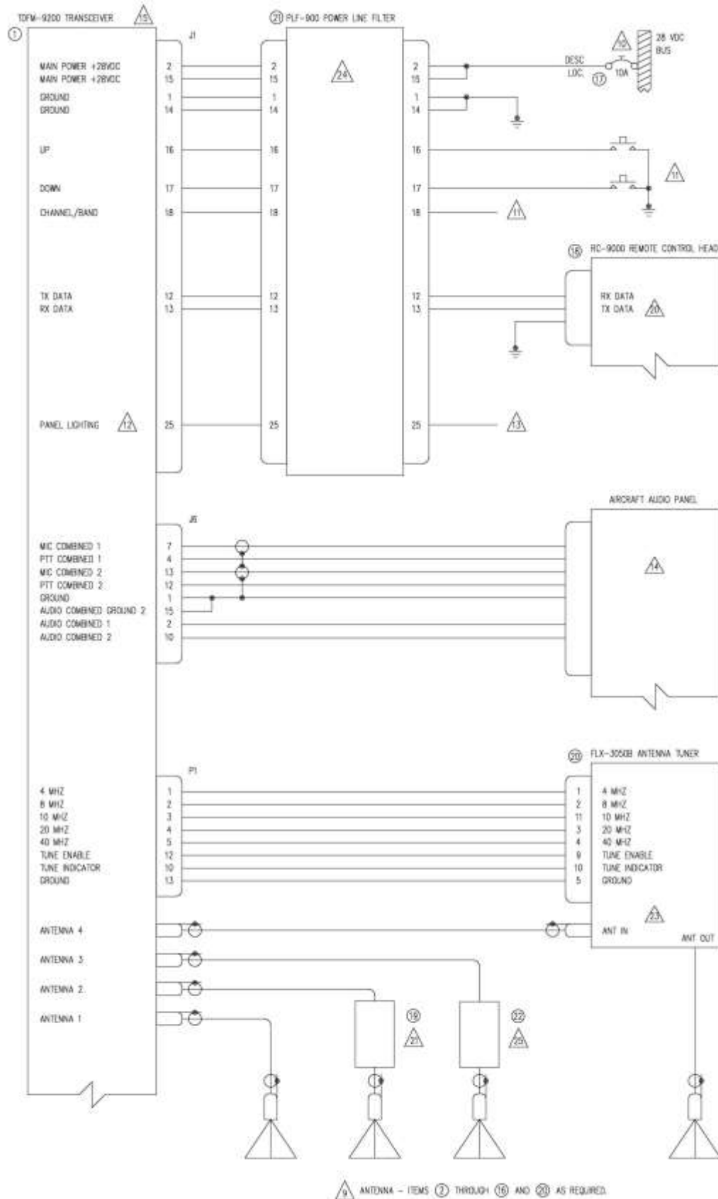
FIGURE 5: Wiring Connections for Combined Band Control.
