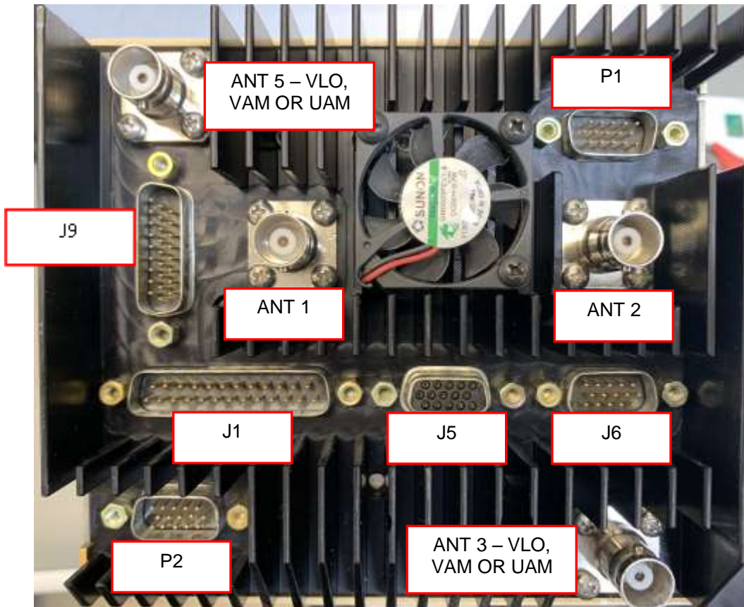
FIGURE 2: TDFM-9200 Antenna & Connector Locations
