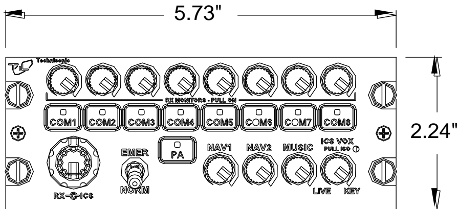
FIGURE 1: Outline Drawing for Model TDAP-650
