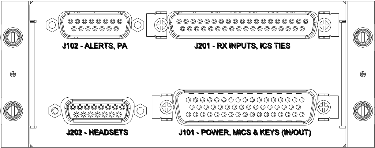
FIGURE 2: TDAP-650 Rear Connectors
