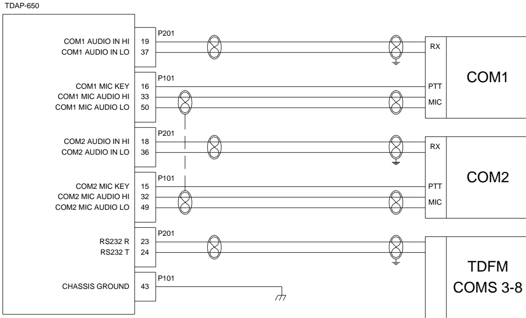
FIGURE 3: Wiring Connections for Communication Transceivers
