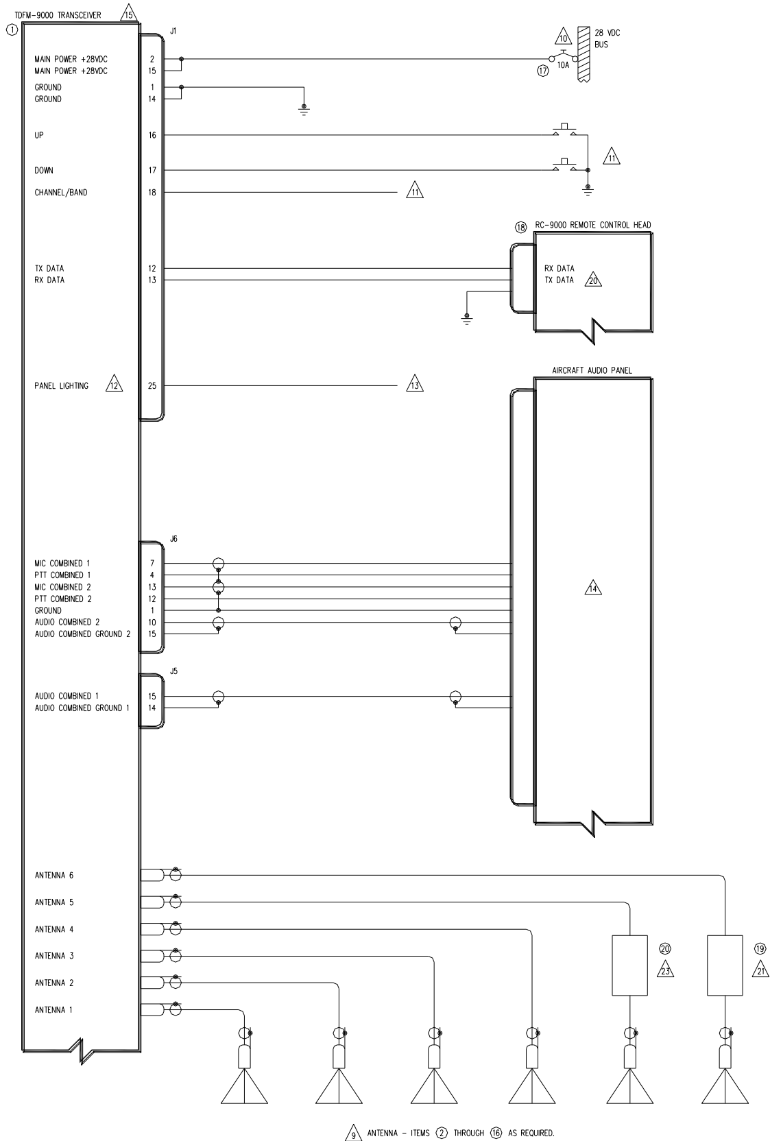
FIGURE 6: Wiring Connections for Combined Band Control with Separate Ground Returns
