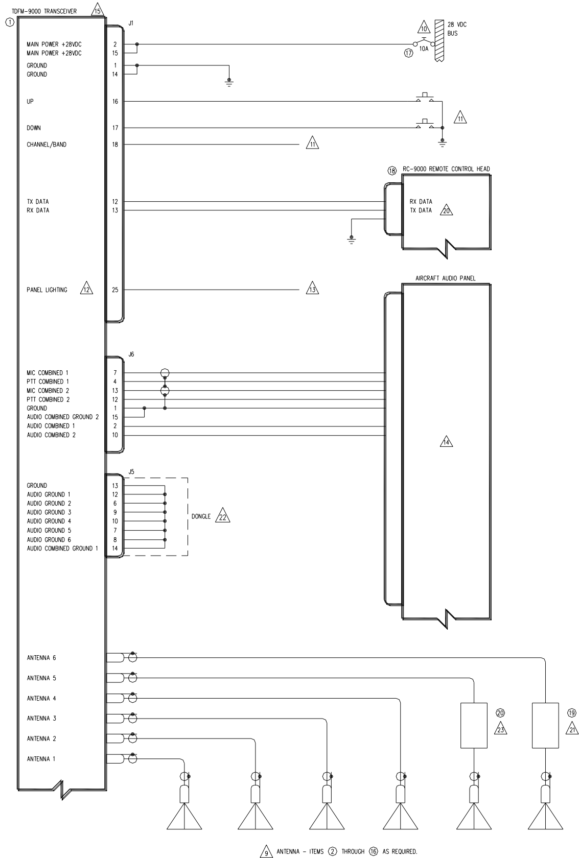
FIGURE 7: Wiring Connections for Combined Band Control with a Single Ground Return
