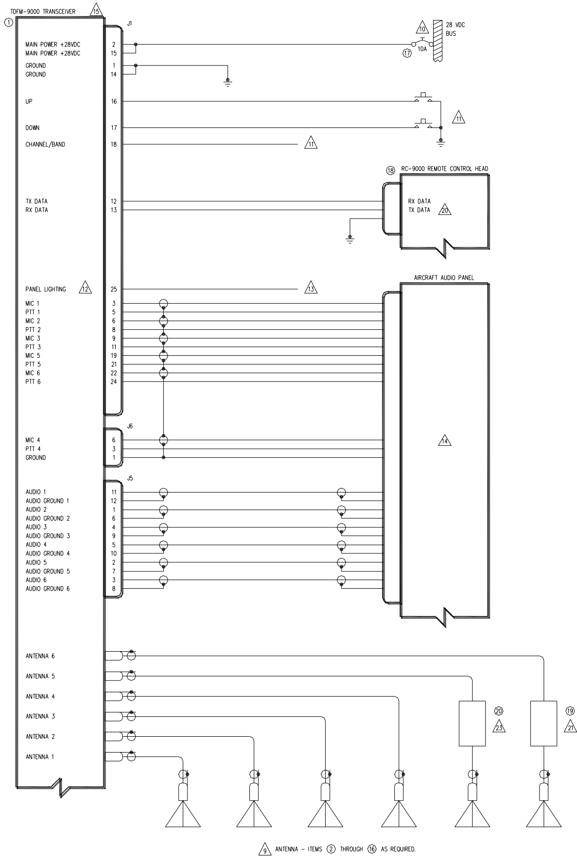
FIGURE 4: Wiring Connections for Individual Band Control with Separate Ground Returns
