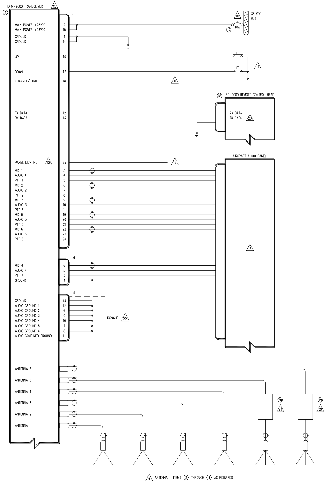
FIGURE 5: Wiring Connections for Individual Band Control with a Single Ground Return
