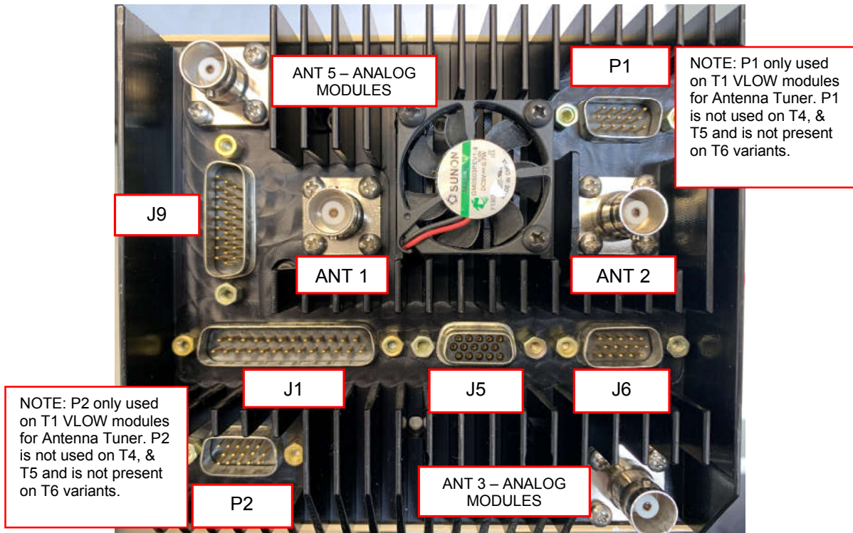
FIGURE 2: TDFM-9200 Antenna & Connector Locations
