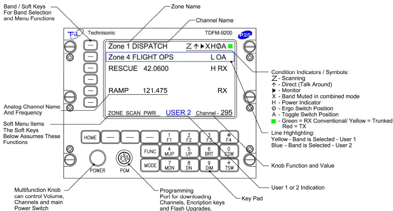
FIGURE 1: Front Panel Controls – TDFM-9200 Transceiver
