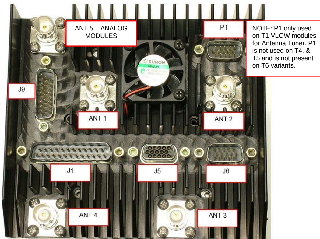
FIGURE 2: TDFM-9300 Antenna & Connector Locations
