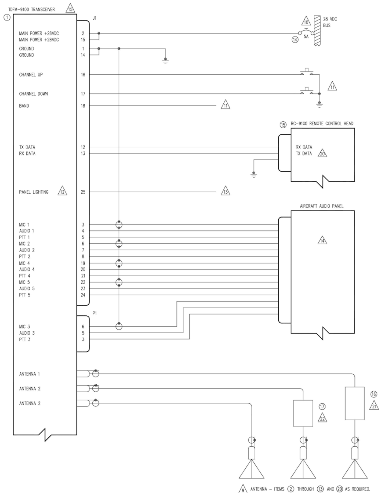
FIGURE 4: Wiring Connections for Separate Band Control
