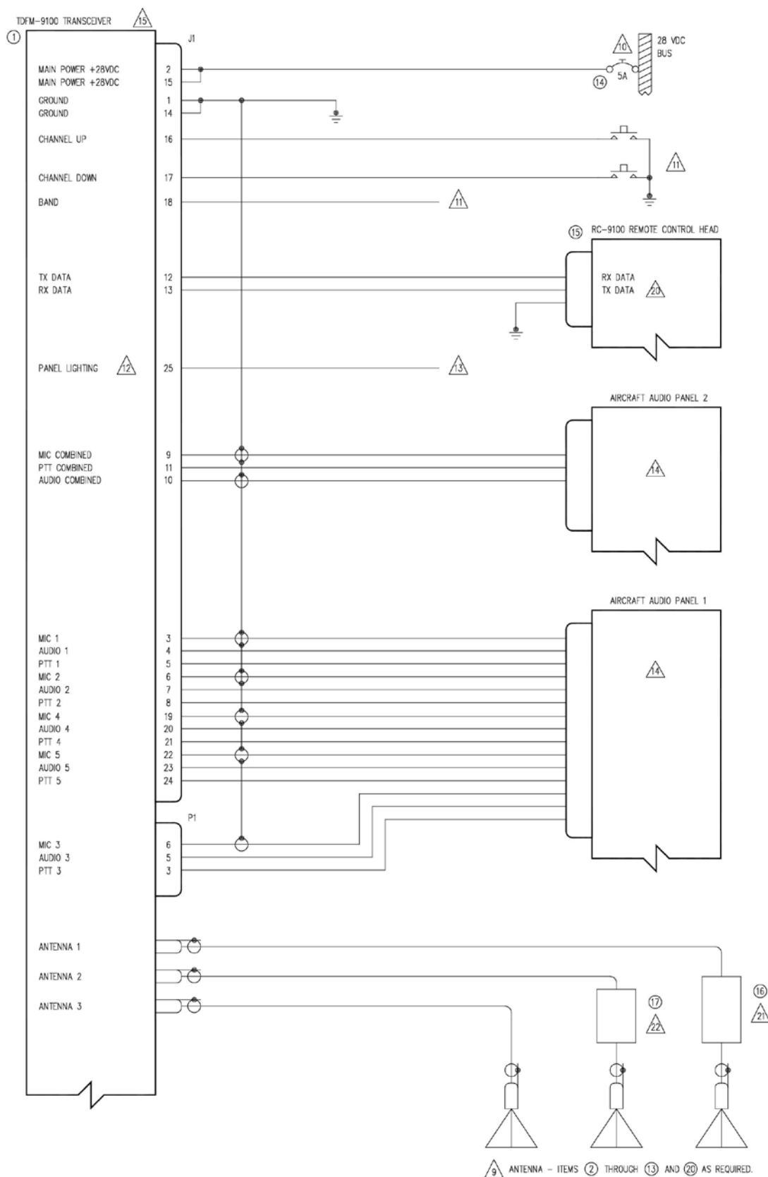
FIGURE 5: Wiring Connections for Combined Band Control
