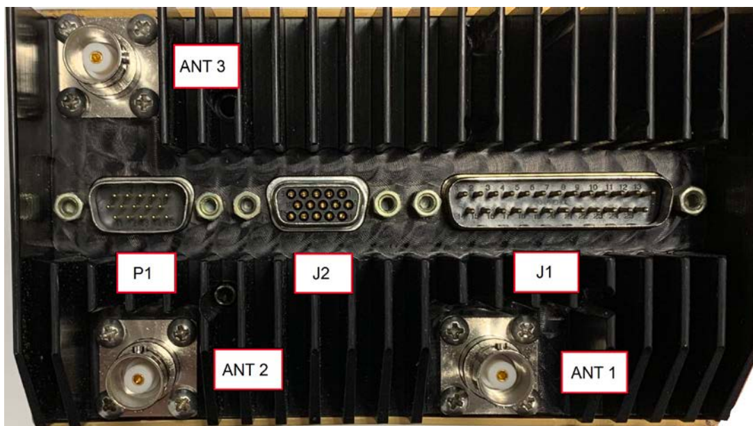
FIGURE 2: TDFM-9100 Antenna & Connector Locations (P1 and J2 on units with MOD 14 only)
