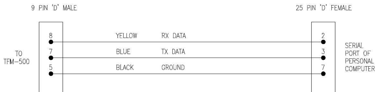
FIGURE 2.2 TFM-530 Transceiver PC Up/Download Cable - wiring diagram
