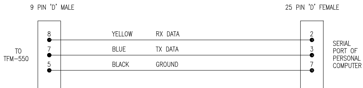
FIGURE 2.2 TFM-550 Transceiver PC Up/Download Cable - wiring diagram
